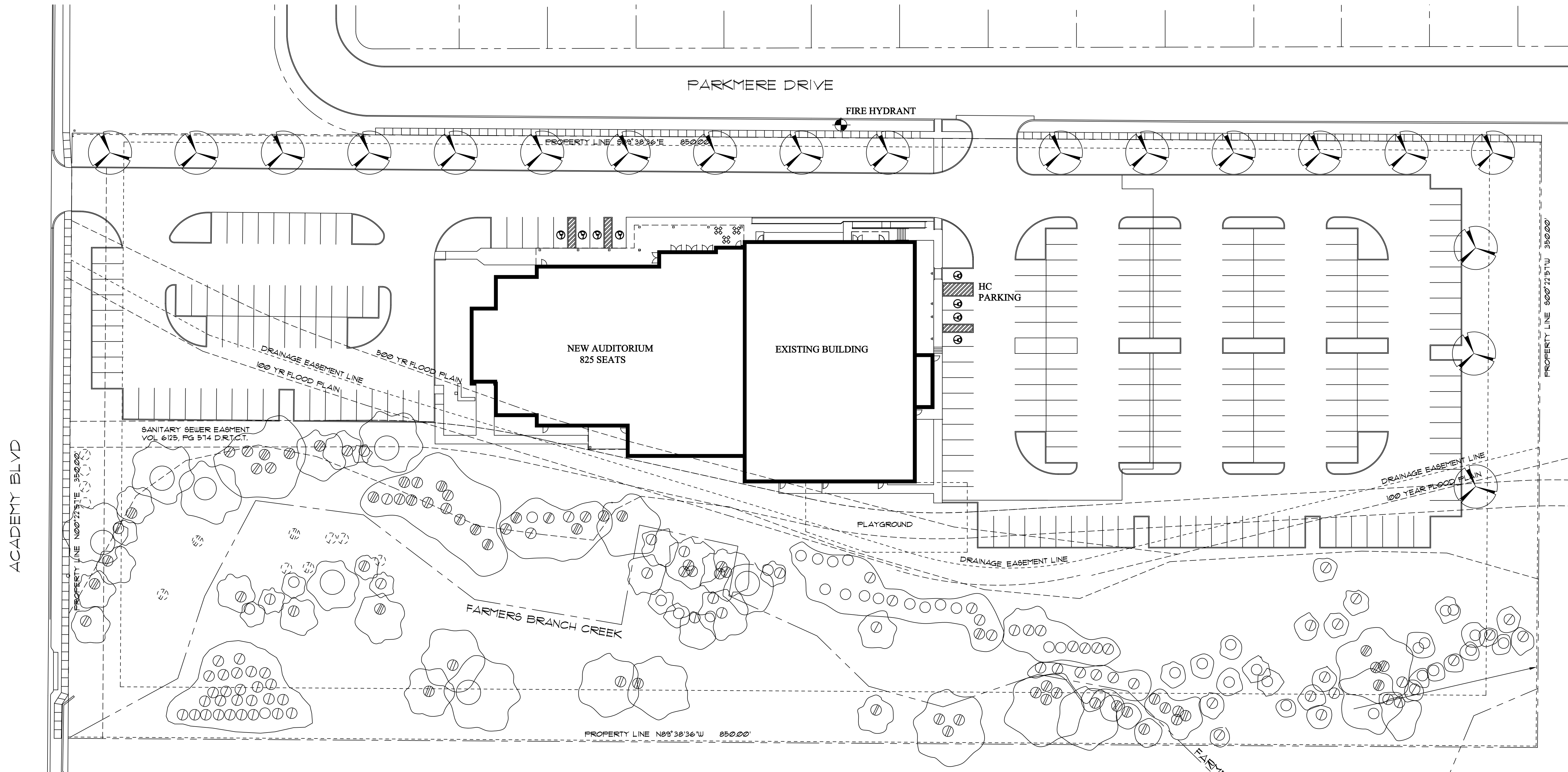
SITE PLAN SCALE: 1" = 30'-0"
